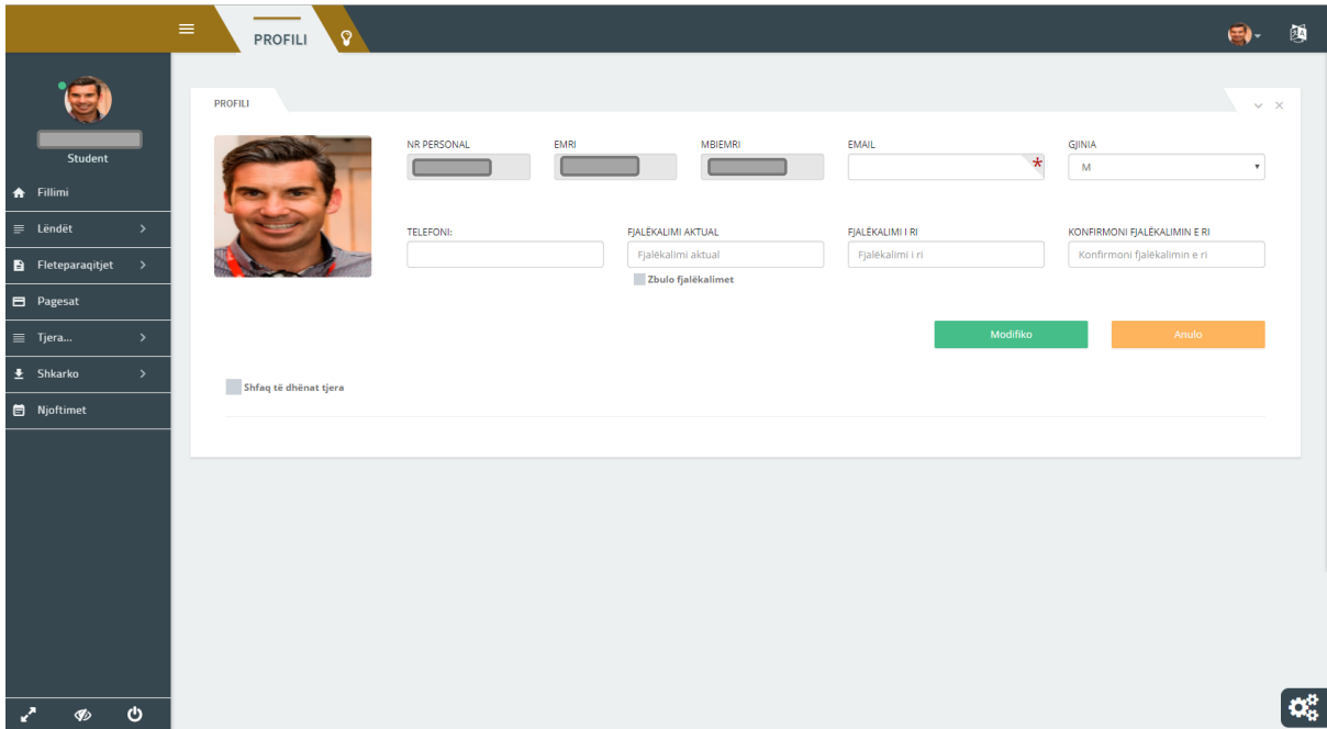
Figure 12: Profili
