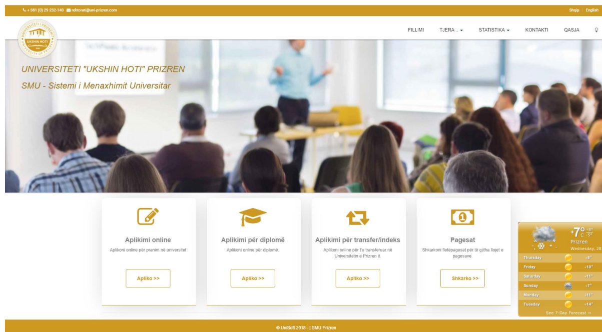
Figure 1: Ballina
