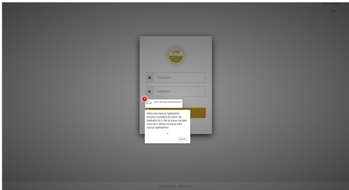
Figure 3: Ndihma
